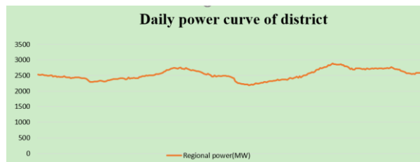
Fig. 4. Daily power load curve of region.
