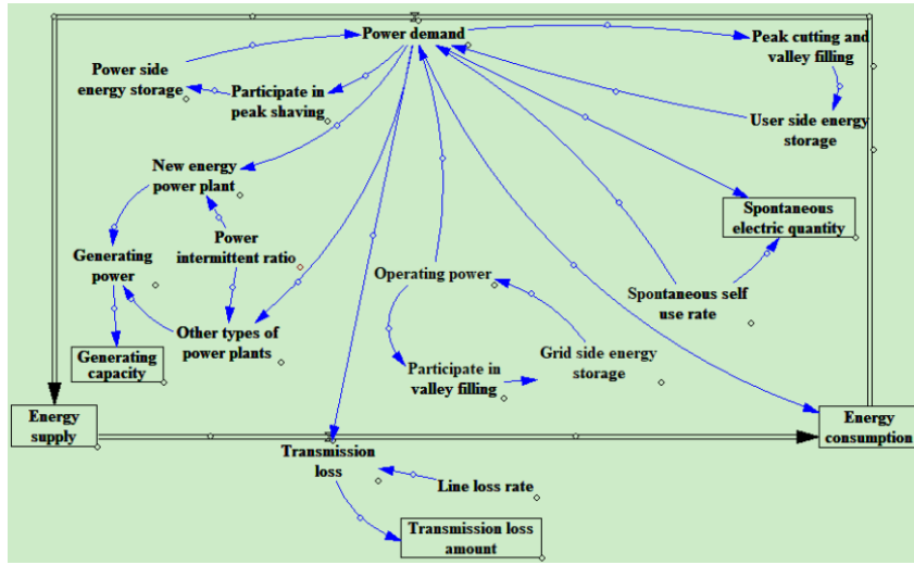
Fig. 3. Dynamic mode of energy supply and demand system with high proportion of renewable energy resources.
